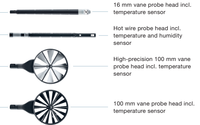
testo 440 probe heads for air velocity incl. temperature and humidity sensor
